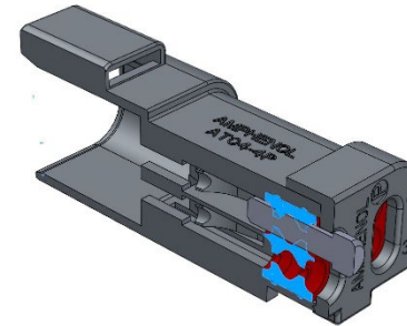
AT Cavity Plug in EC Section
