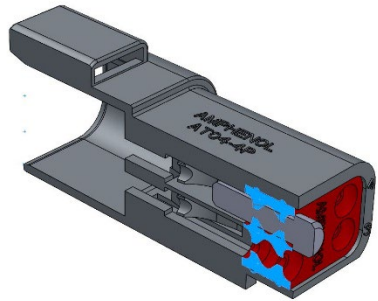
AT Cavity Plug Section
