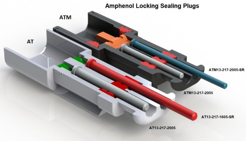
AT Cavity Plug in SR Section
